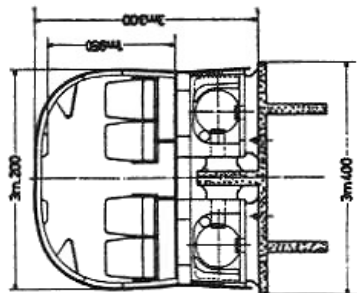
SECTION CC Version confort
